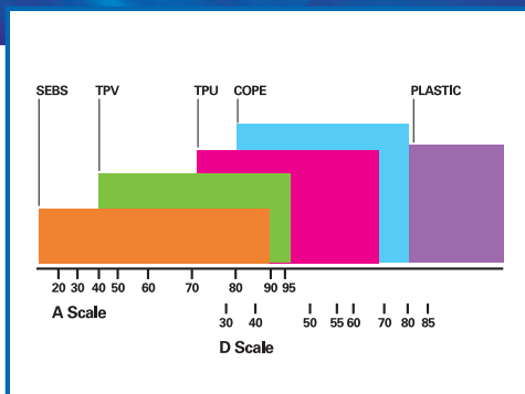
Durometer Scale
