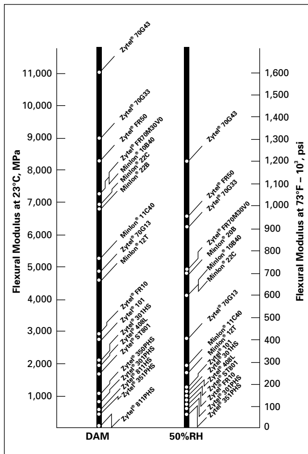
Figure 44. Flexural Modulus at 23°C (73°F), Comparison Charts
