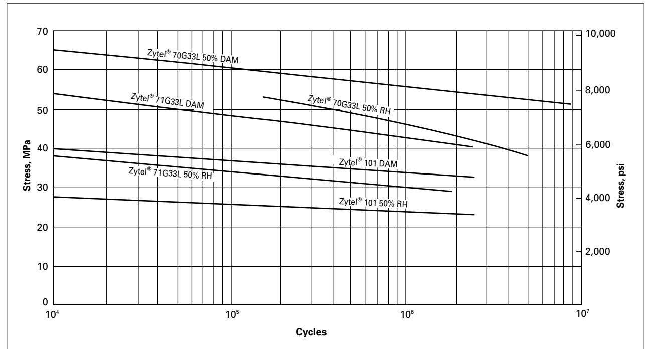
Figure 91. Fatigue Resistance, Tension-Compression 1800 Cycles/min, GRZ vs. Zytel® 101
