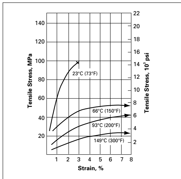
Figure 12. Stress-Strain for Minlon® 10B40, DAM at Four Temperatures
