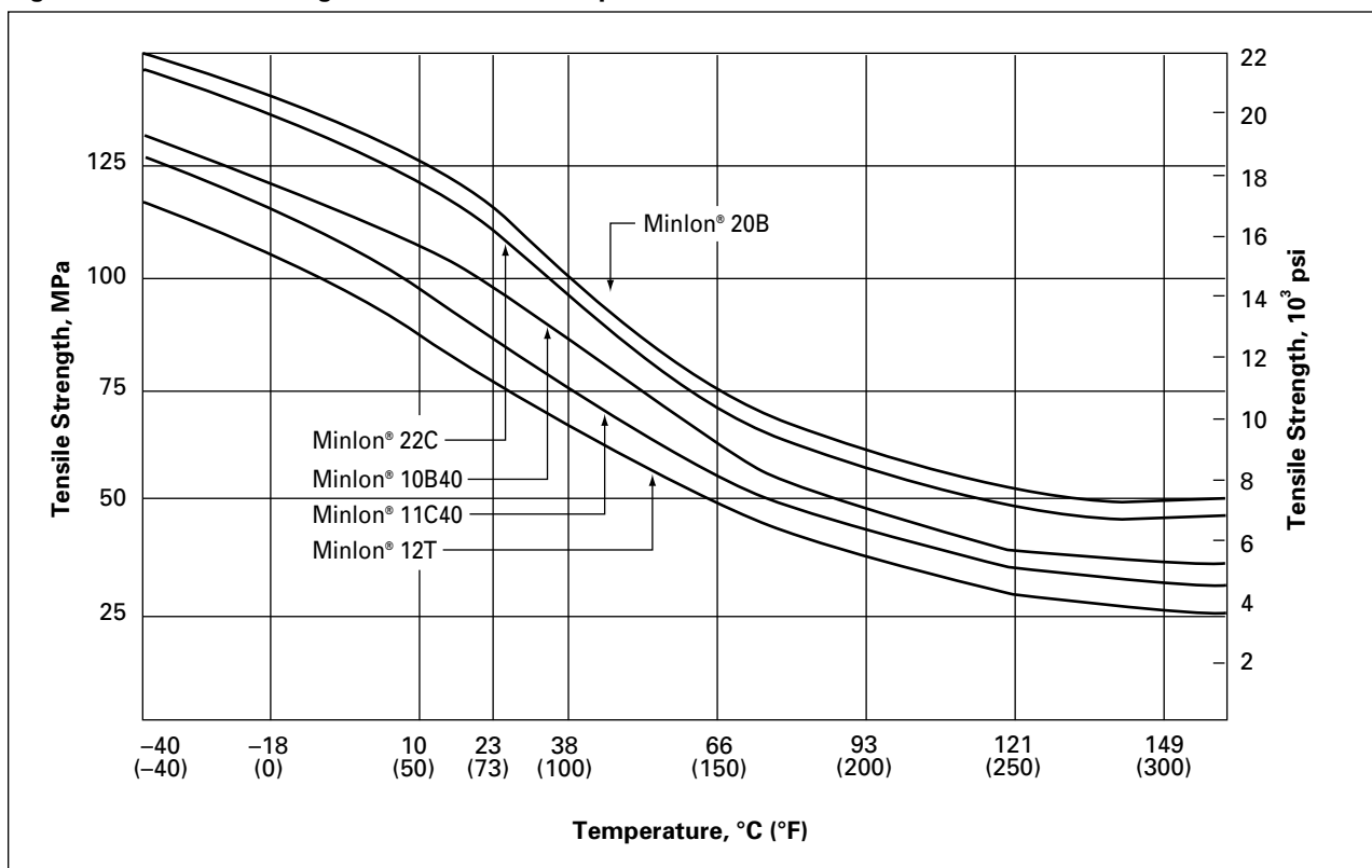
Figure 24. Tensile Strength of Minlon® vs. Temperature, DAM
