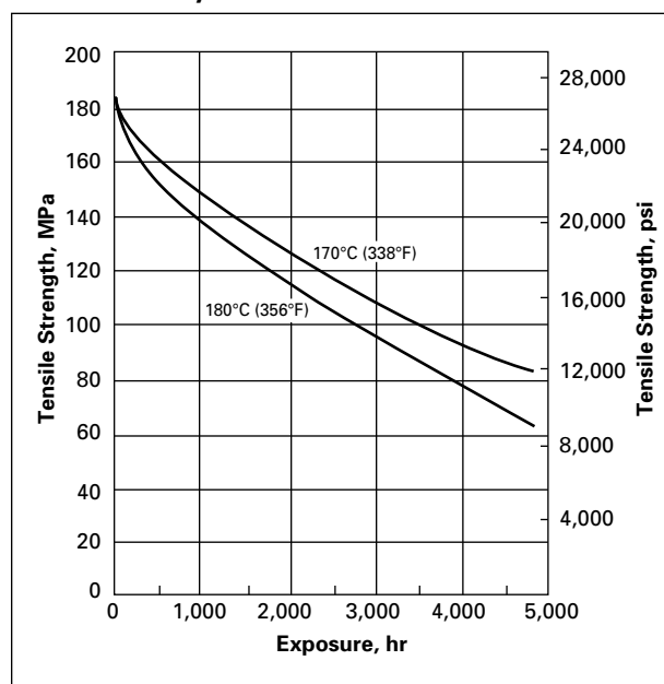
Figure 141. Effect of Air Oven Aging at Different Temperatures on Tensile Strength of Zytel® 77G43L
