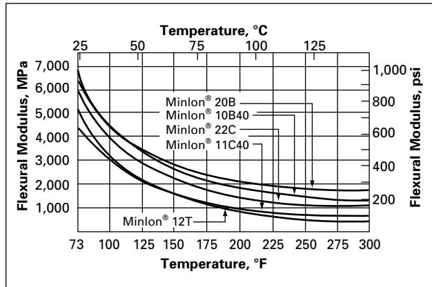
Figure 53. Flexural Modulus of Minlon® vs. Temperature, DAM
