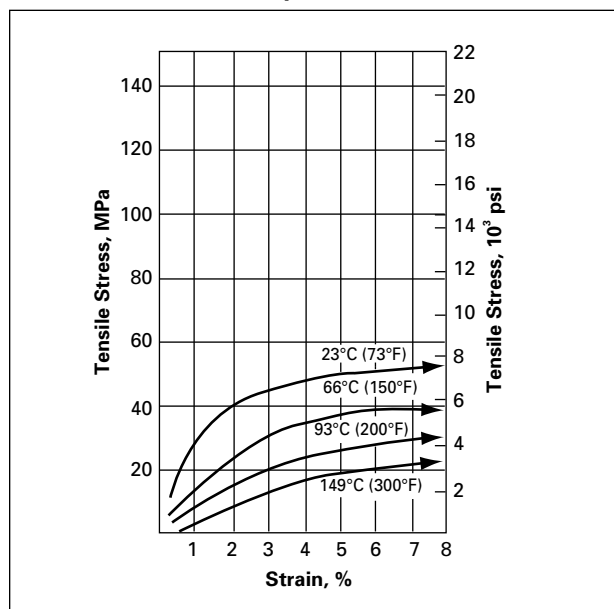
Figure 13. Stress-Strain for Minlon® 10B40, 50% RH at Four Temperatures
