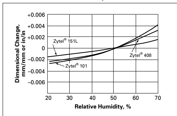
Figure 122. Dimensional Change as a Function of Cyclic Variations in Environmental Relative Humidity
