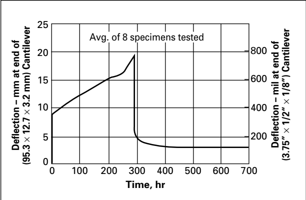
Figure 84. Cyclic Loading and Recovery of Zytel® 101, Long Term, 20.7 MPa (3,000 psi), 23°C (73°F)
