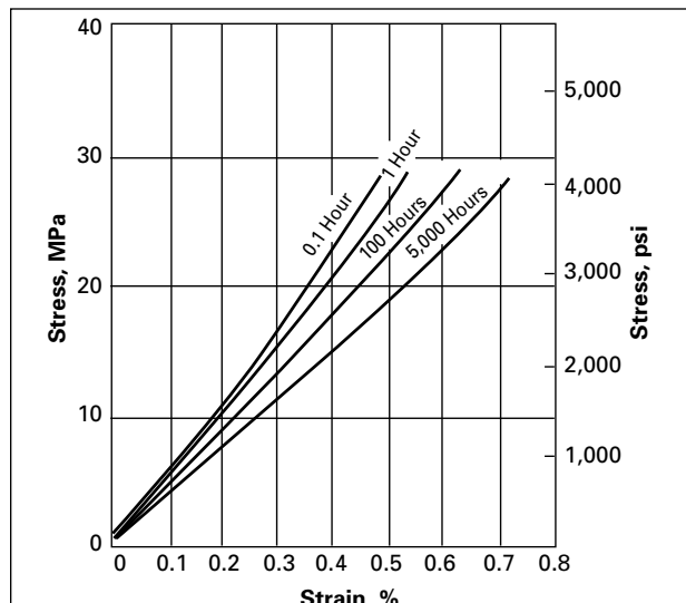
Figure 64. Isochronous Stress vs. Strain Zytel® 70G33L at 23°C (73°F), 50% RH
