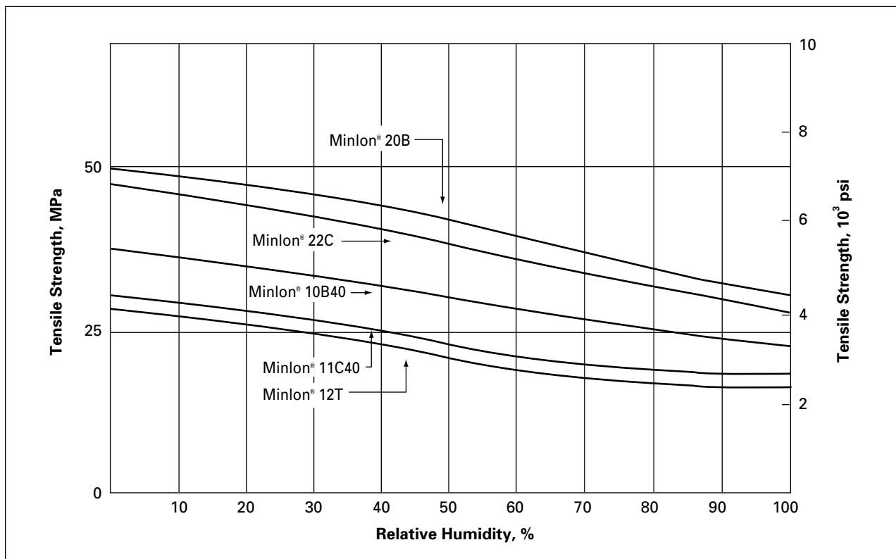
Figure 23. Tensile Strength of Minlon® vs. Humidity at 149°C (300°F)
