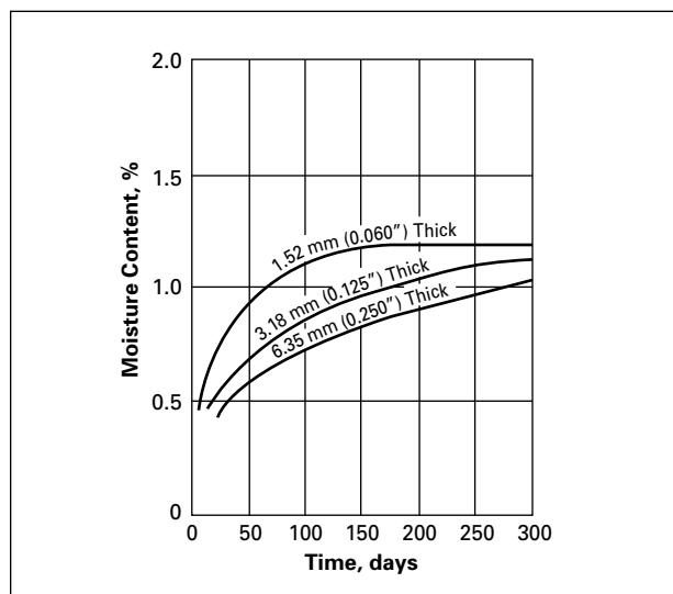
Figure 119. Moisture Content vs. Time for Zytel® 151L Exposed to 50% RH Air at 23°C (73°F)
