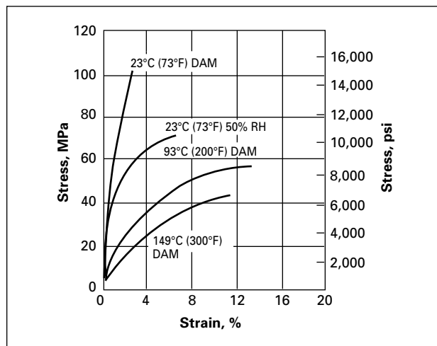
Figure 25. Stress vs. Strain at Three Temperatures, Zytel® 70G13L
