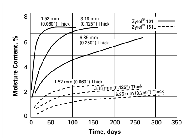
Figure 120. Moisture Content vs. Time for Zytel® 101 and Zytel® 151L Immersed in Water at 23°C (73°F)
