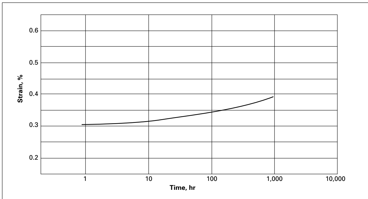
Figure 76. Creep in Flexure of Minlon® 20B at 6.9 MPa (1,000 psi), 124°C (257°F), DAM
