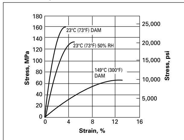
Figure 30. Stress vs. Strain at Two Temperatures, Zytel® 77G33L
