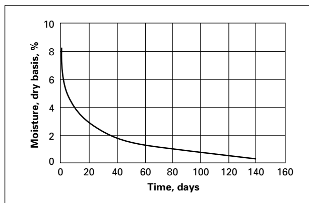
Figure 121. Rate of Moisture Loss, Zytel® 101, 23°C (73°F), Over Drierite®, 1.6 mm (1/16\"/>
