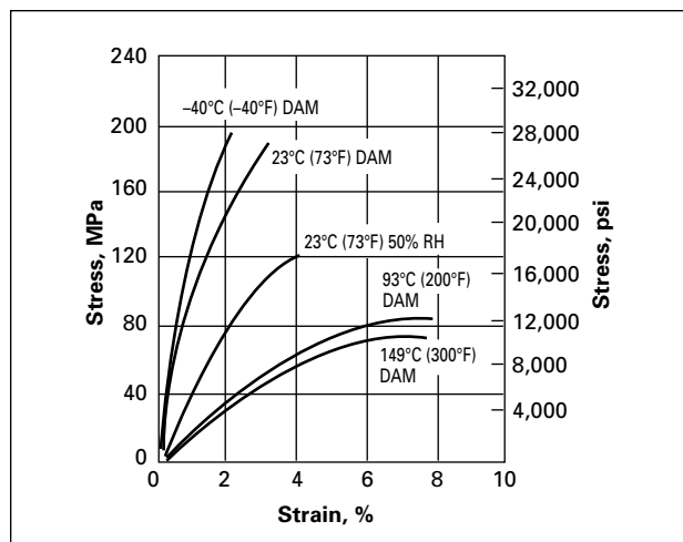
Figure 26. Stress vs. Strain at Four Temperatures, Zytel® 70G33L
