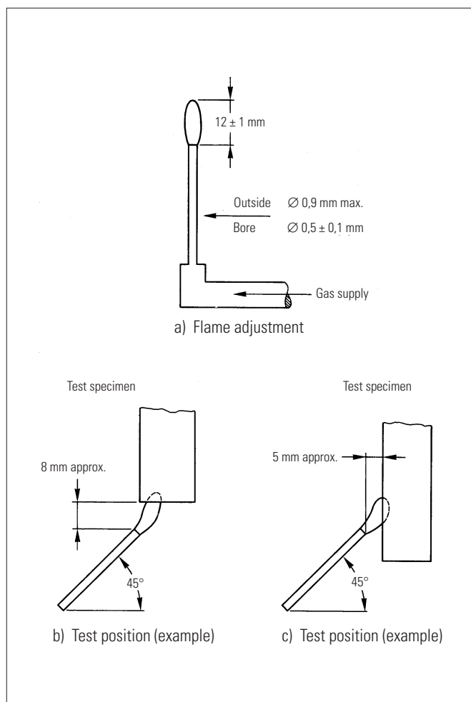
Fig. 1. Needle burner
