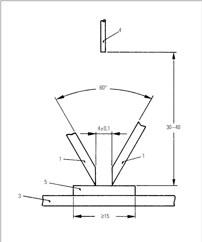
Fig. 2. Electrode arrangement a)
