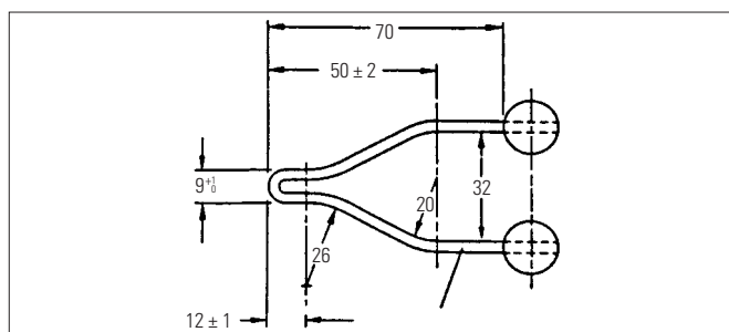
Fig. 1. Glow-wire
