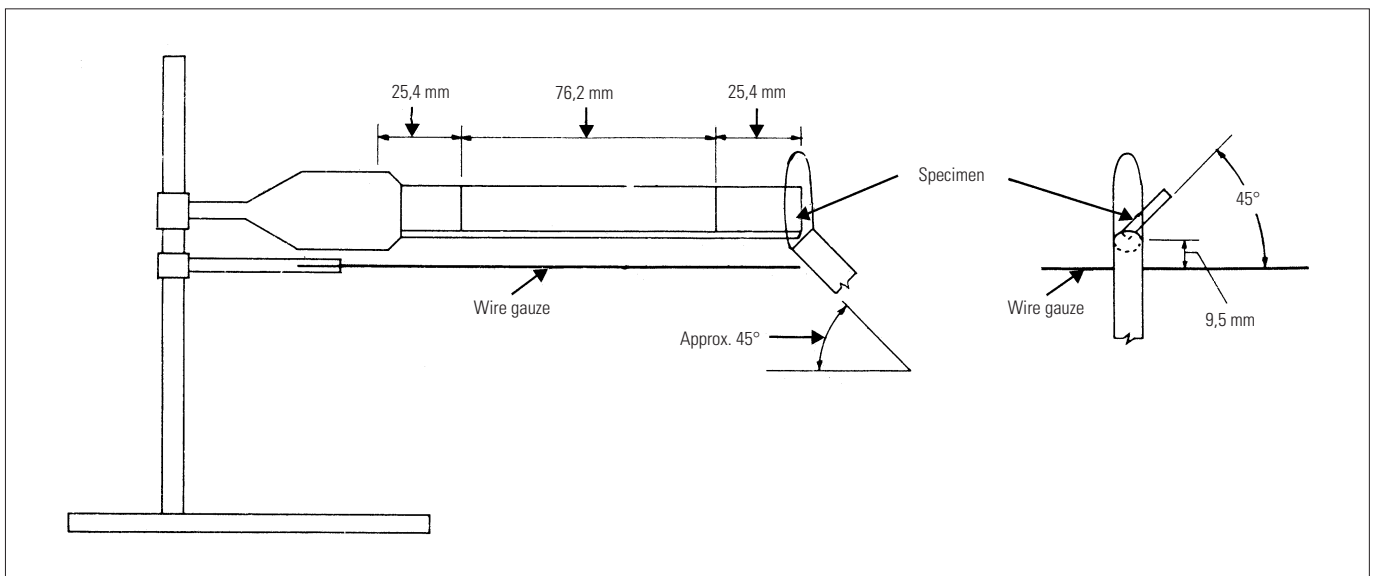
Fig. 1. Horizontal burning test for 94 HB classification
