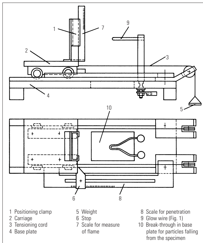
Fig. 2. Test equipment
