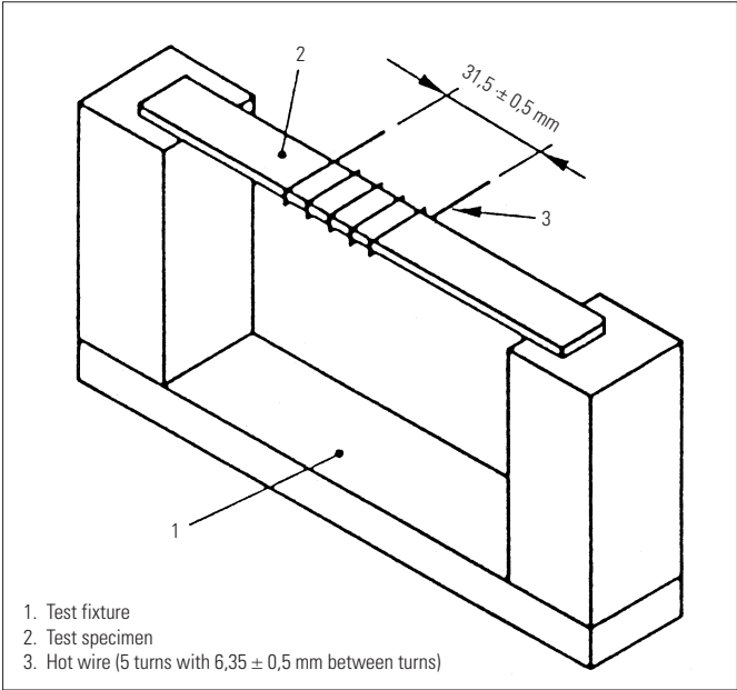
Fig. 1. Method B: Hot-wire coil ignition. Test apparatus (example)
